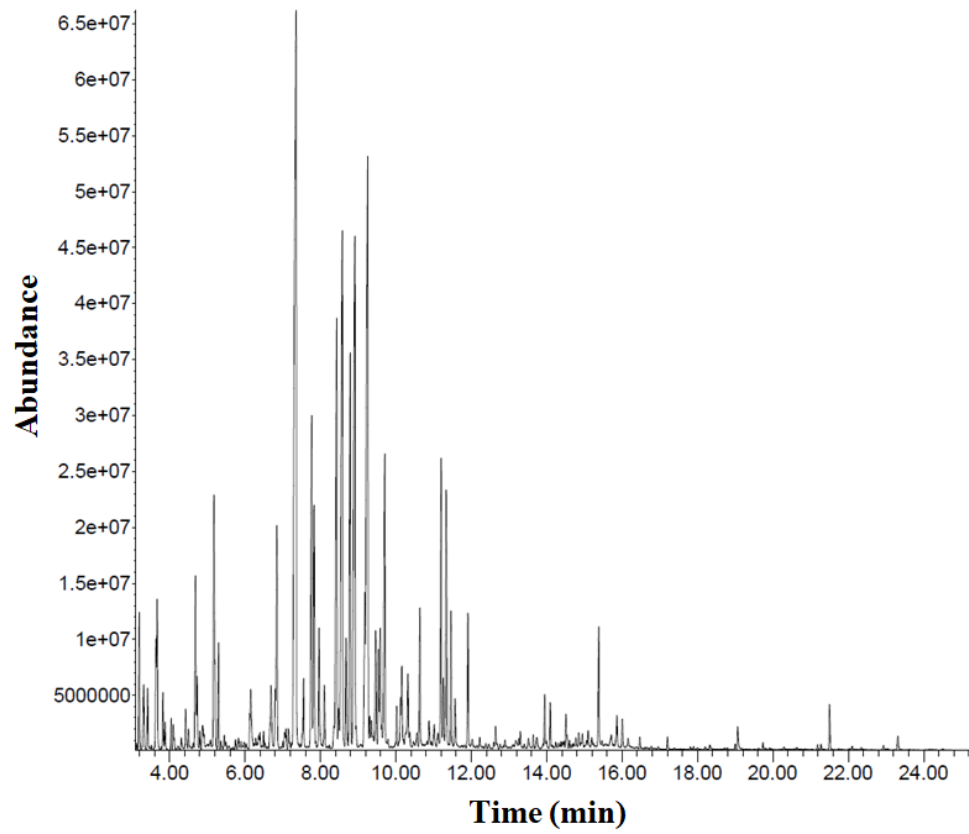
Supplementary Figure 1. Chromatograms of essential oil obtained from Abeliophyllum distichum flowers
